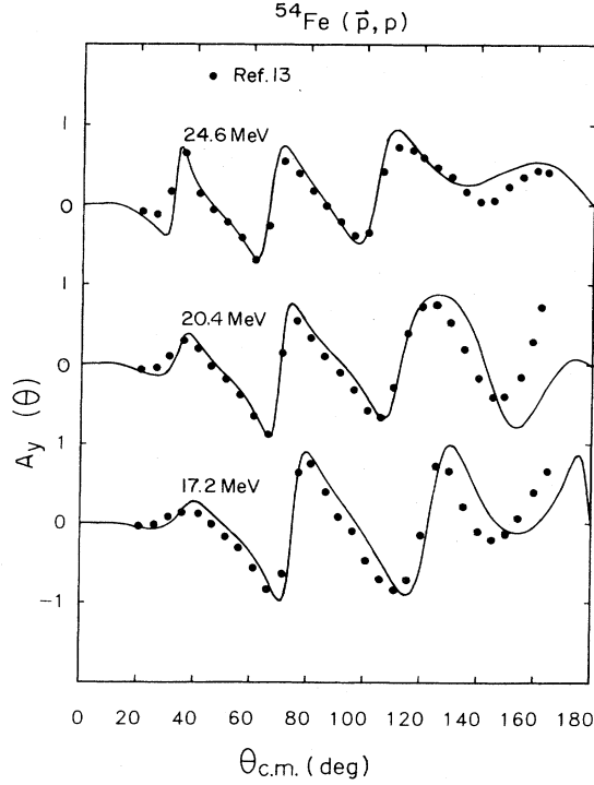
FIG. 7. Brieva-Rook microscopic optical model calculations are compared to measured analyzing powers for ^{54}\text{Fe}(\bar{p}, p) .
