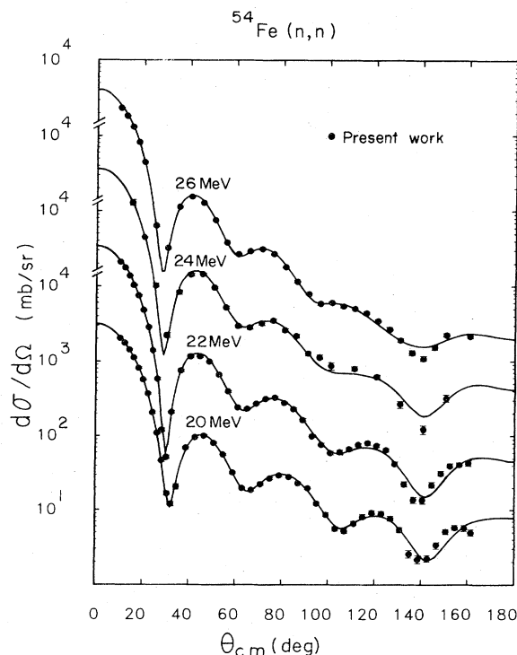
FIG. 1. Average geometry phenomenological optical model fits are compared to measured cross sections for ^{54}\text{Fe}(n,n) . Optical parameters are given in Table I.
