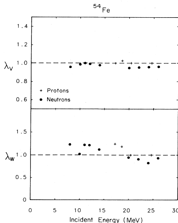
FIG. 11. Normalizing parameters for JLM optical potentials.
