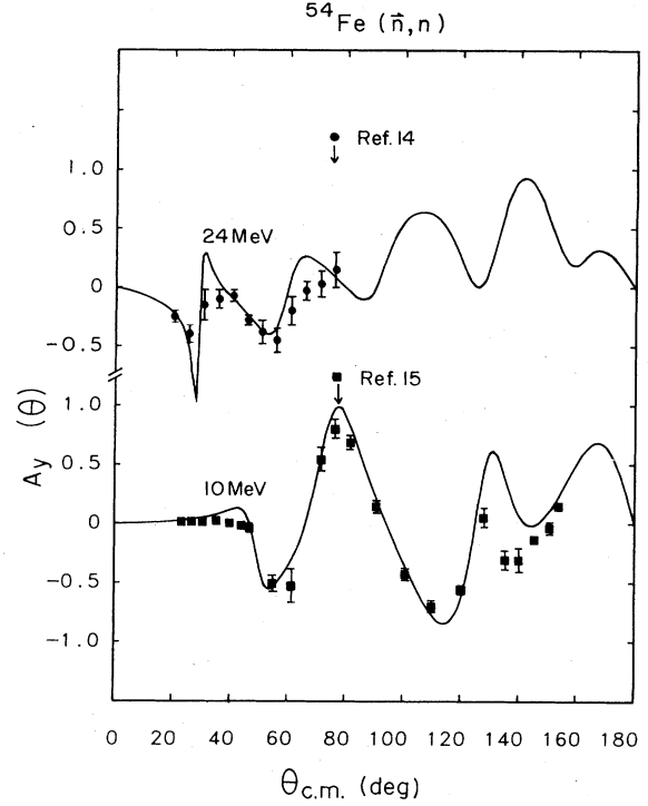
FIG. 8. Brieva-Rook microscopic optical model calculations are compared to measured analyzing powers for ^{54}\text{Fe}(\bar{n}, n) .
