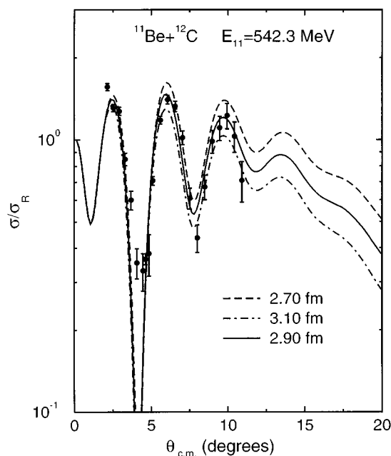
FIG. 5. Calculated ^{11}\text{Be} + ^{12}\text{C} elastic cross-section angular distributions (ratio to Rutherford) at 49.3 MeV/nucleon for projectile wave functions with rms matter radii of 2.70 fm (long-dashed curve), 2.90 fm (solid curve), and 3.10 fm (dot-dashed curve).
