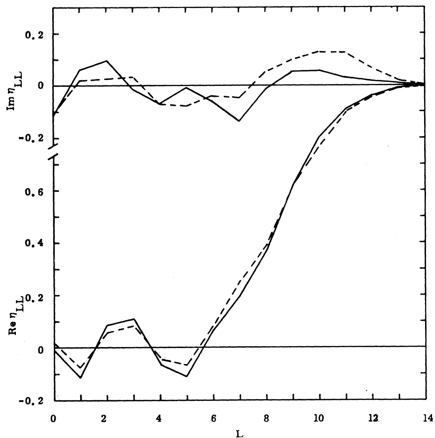
FIG. 10. Reflection coefficients \eta_{LL} for d+\text{Ni} at E_d=21.6 MeV. The solid curve is generated by V_{PH} and the dashed curve is generated by the coupled equation (38) with V_{00} replaced by 0.9 \text{ Re}(V_{00}) + i \text{Im}(V_{00}) .
