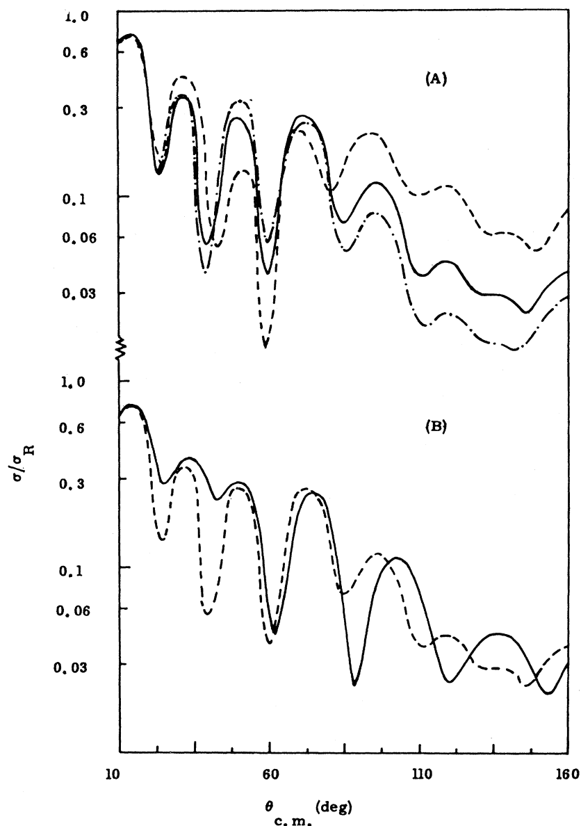
FIG. 8. (A) Changes in the differential cross sections (for d+Ni at E_d=21.6 MeV) generated by V_{00} (no coupling) when the real part of V_{00} is multiplied by 1.0 (dashed curve), 0.9 (solid curve), and 0.86 (dashed-dot curve). (B) Comparison between the cross section generated by V_{PH} (solid curve) and the cross section obtained when \text{Re } V_{00} is multiplied by 0.9 (dashed curve).
