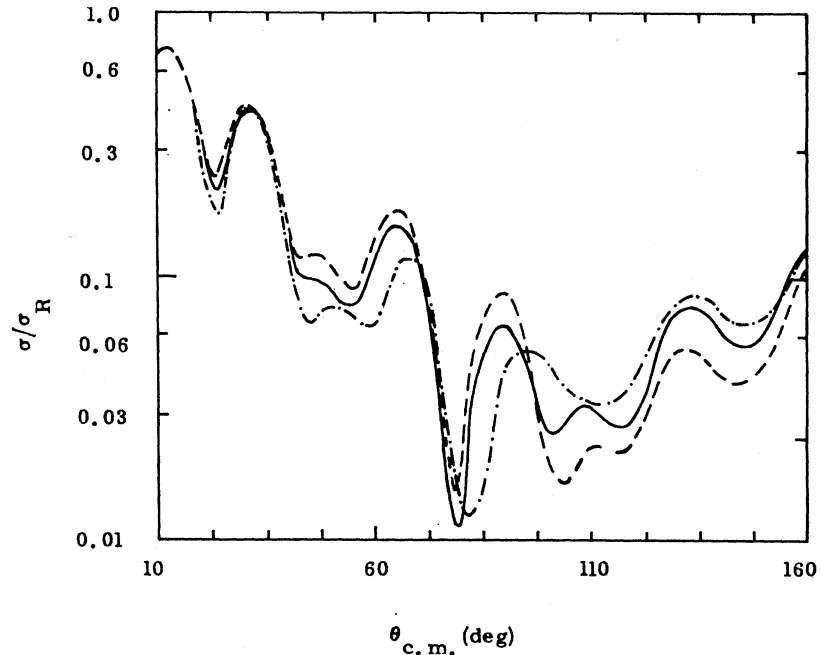
FIG. 7. Differential cross sections for d+\text{Ni} at E_d=21.6 MeV generated by the coupled equations with \bar{\epsilon}_k=2.5 MeV (dashed curve), \bar{\epsilon}_k=5 MeV (solid curve), and \bar{\epsilon}_k=10 MeV (dashed-dot curve).
