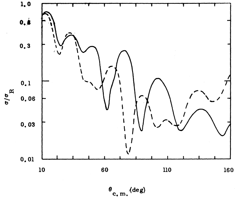
FIG. 6. Differential cross sections for d+\text{Ni} at E_d=21.6 MeV. The solid curve is generated by V_{PH} and the dashed curve by the coupled equations (with \bar{\epsilon}_k=5 MeV).
