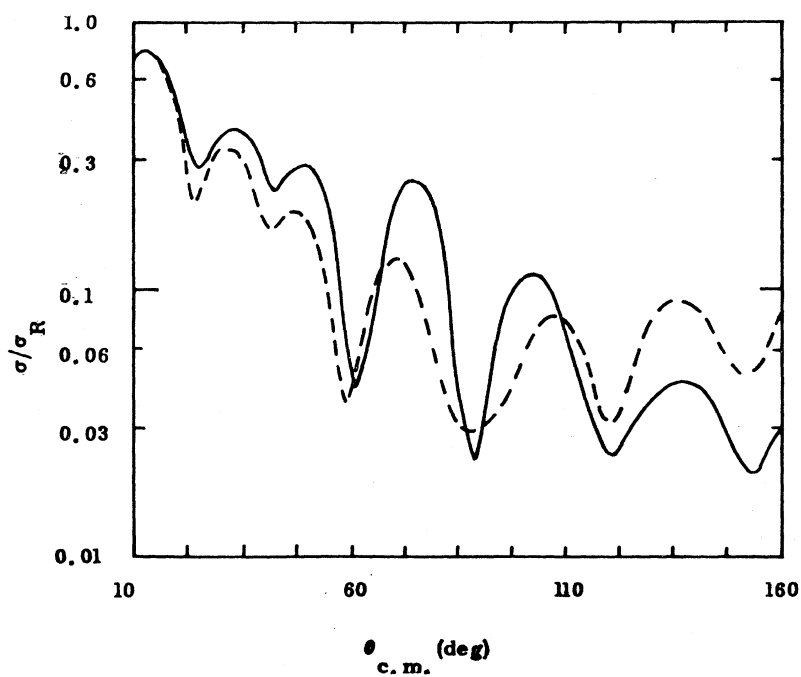
FIG. 11. Differential cross sections d+\text{Ni} at E_d=21.6 MeV generated by V_{PH} (solid curve) and the coupled equations with V_{00} modified as in Figs. 9 and 10.
